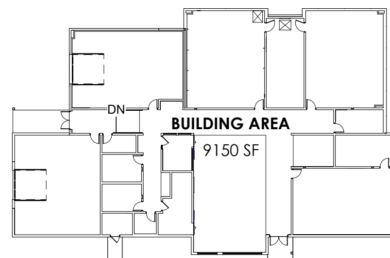
2 KEY PLAN - FIRST FLOOR 1/32" = 1'-0"
